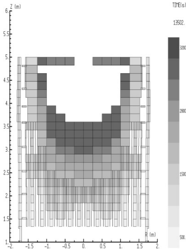
Fig. 23. Calculation with the radiative conductivity model; time = 13500 s.
