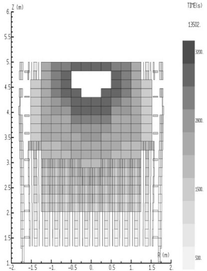
Fig. 24. Calculation with the Hottel model; time = 13500 s.
