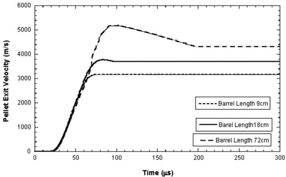
Fig. 6. Time history of the pellet velocity for the 9, 18 and 72cm barrels.
